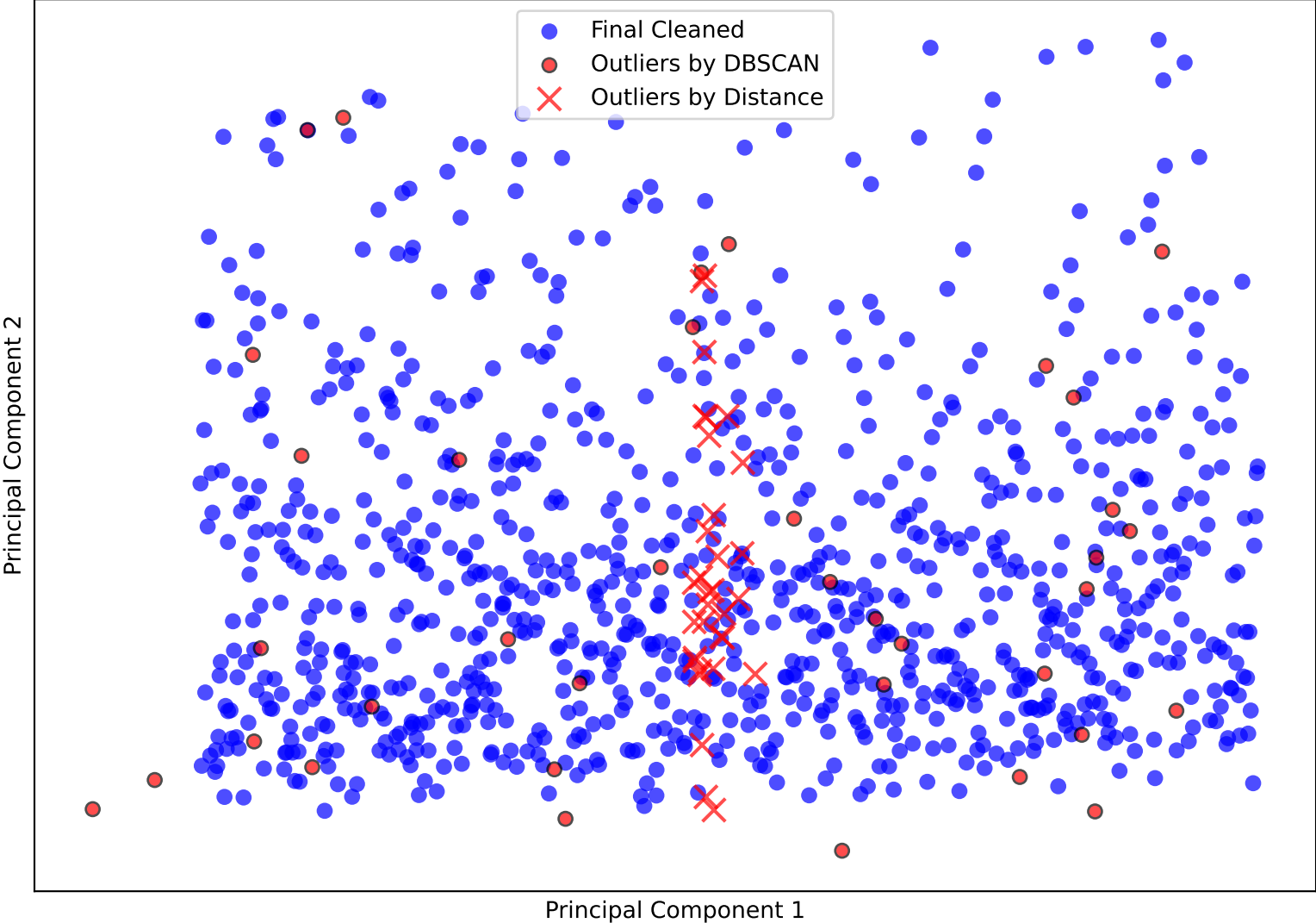
German Credit: PCA-Reduced Scatter Plot of Data Points and Outliers
